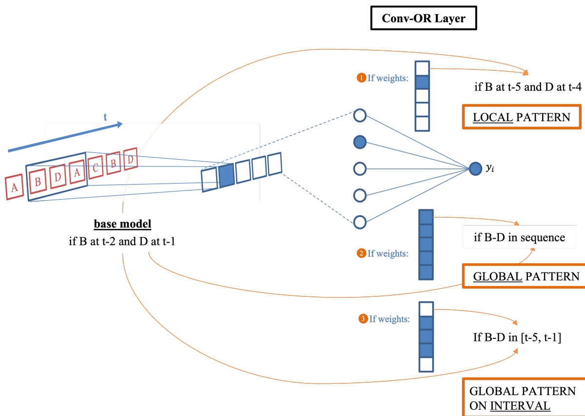
Figure 1: Architecture of the model with an example on a sequence of letters. The base rule model is applied as 1D-convolutional window over the sequence. The resulting boolean values are given as input of the Conv-OR layer which indicates through its activated weights where along the sequence the expression learned by the base model is true. The output of the Conv-OR layer is mapped to the label of the sequence y_i . For local patterns, the base model expression needs to be shifted accordingly to the Conv-OR Layer weights.
